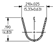
SECT. "A-A"
