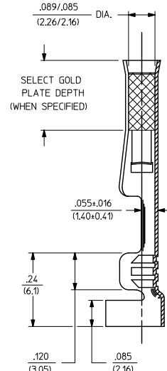
SECT. "C-C"
