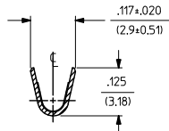
SECT. "B-B"
