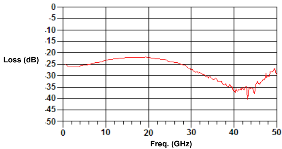
Output Return Loss (Insertion Loss State)
