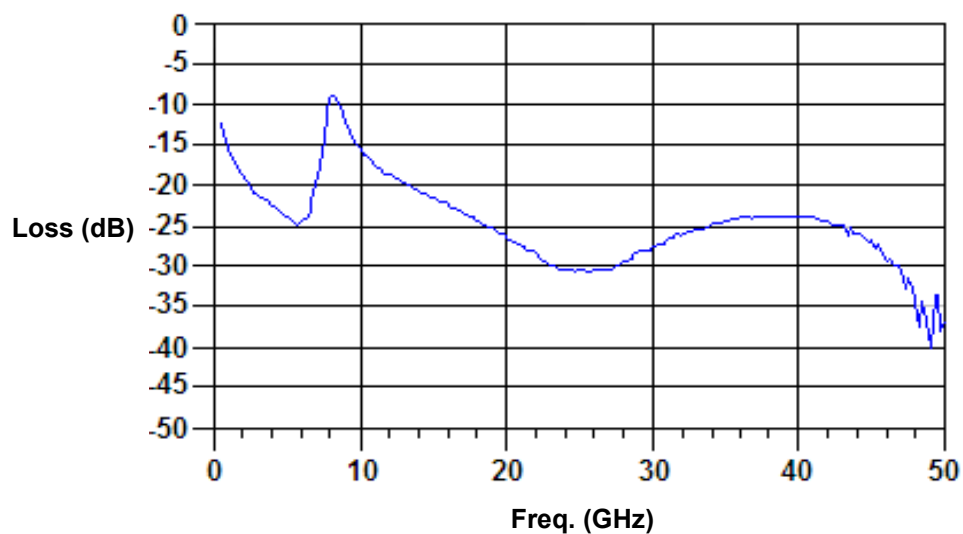
Output Return Loss (Isolation Loss State)
