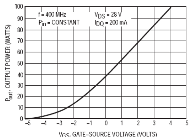
Figure 4. Output Power versus Gate Voltage
