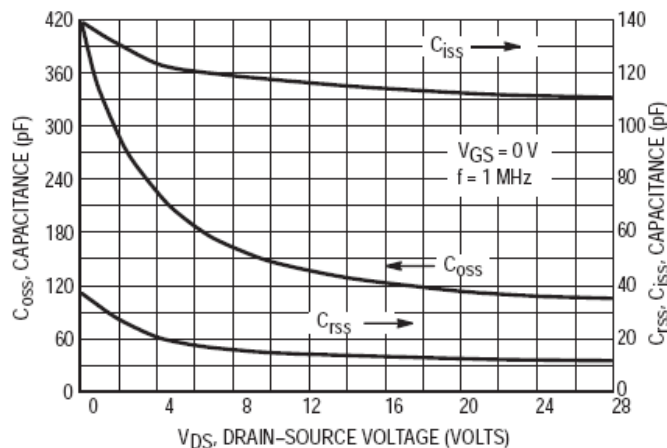
Figure 5. Capacitance versus Drain Voltage
