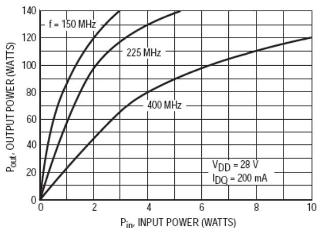
Figure 1. Output Power versus Input Power
