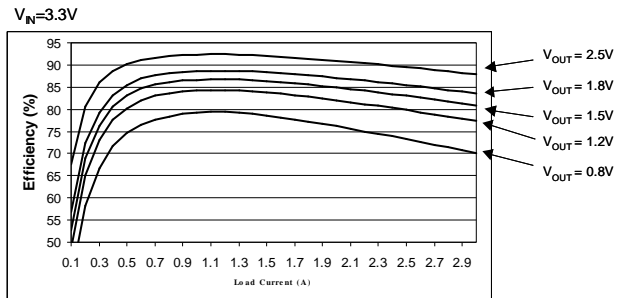
Efficiency versus Load, V_{IN} = 3.3V
