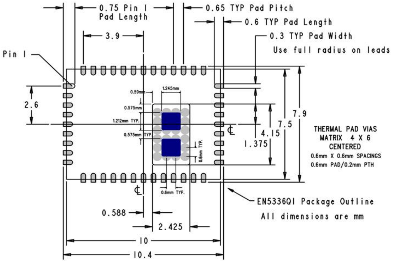
Figure 6: EN5336QI PCB Footprint (Top View)
