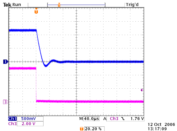
Shut-down waveform, V_{IN}/V_{OUT} = 5.5V/1.2V
