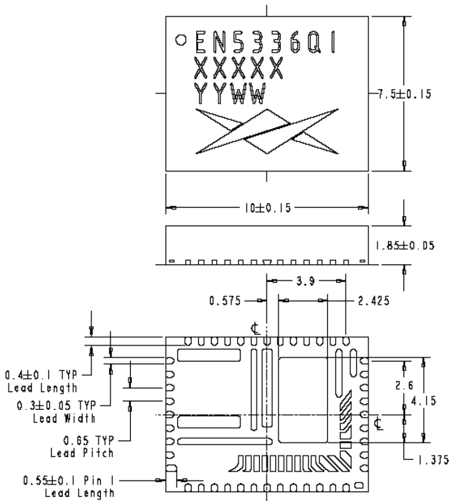
Figure 7. Package dimensions.
