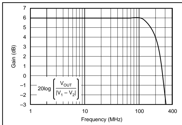
FIGURE 4. High-Speed Instrumentation Amplifier Response.
