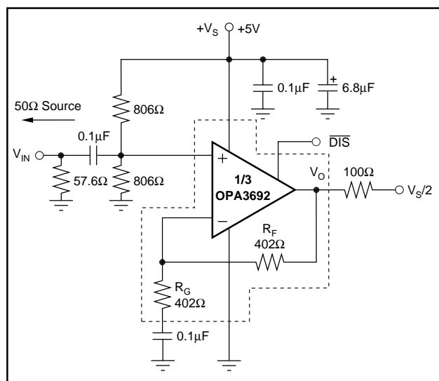
FIGURE 2. AC-Coupled, G = +2 , Single-Supply Specification and Test Circuit.
