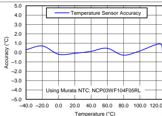
Figure 3. Temperature Accuracy
