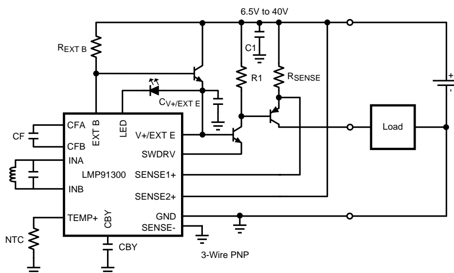
Figure 20. 3-Wire PNP Configuration
