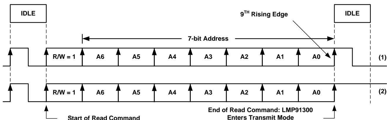
Figure 17. Read Timing Example: (1) Single Pulse, (2) Hold Signal High After Last Rising Edge
