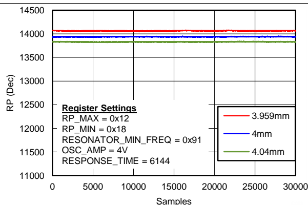
Figure 2. R_p Resolution
