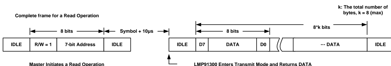
Figure 18. Complete Frame For A Read Command
