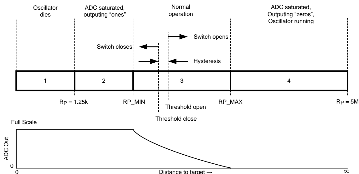
Figure 14. Operating Region
