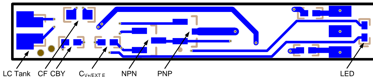
Figure 28. LMP91300 PNP Layout Example
