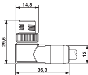
Dimensioned drawing
