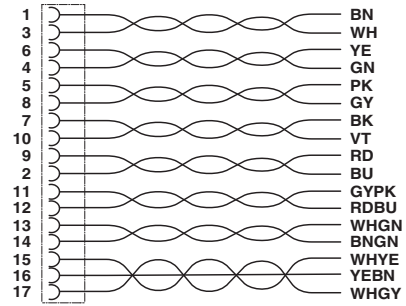
Circuit diagram
