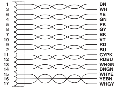
Circuit diagram
