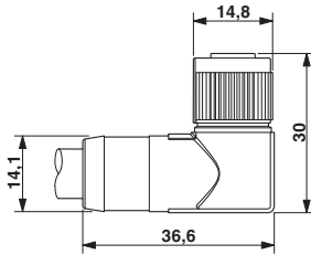
Dimensioned drawing
