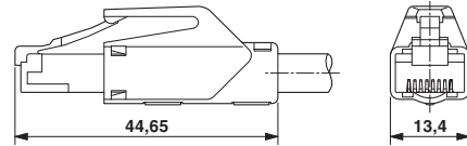
Dimensioned drawing
