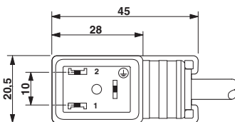
Valve connector, type B
