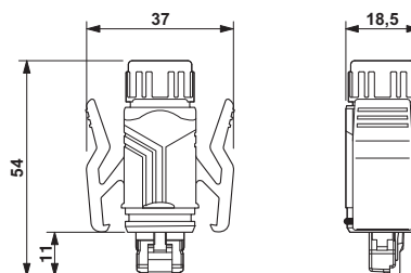
RJ45-connector, IP67
