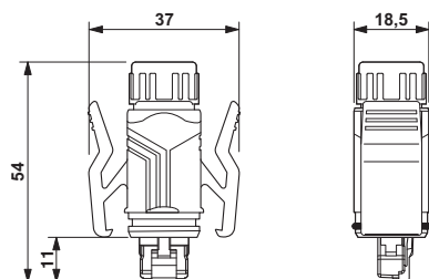
RJ45-connector, IP67
