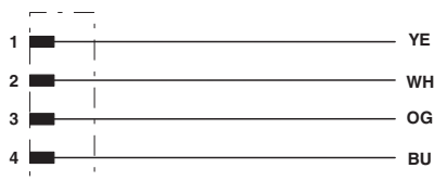
Circuit diagram
