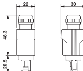
RJ45 Push-Pull connector, IP67
