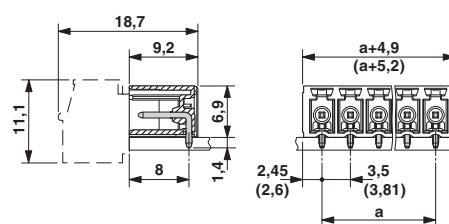
Dimensioned drawing
