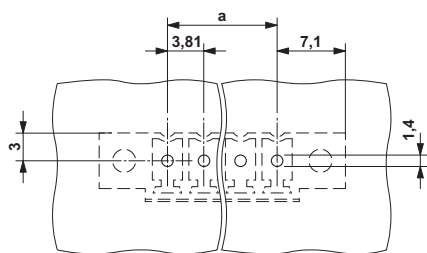
Drilling diagram
