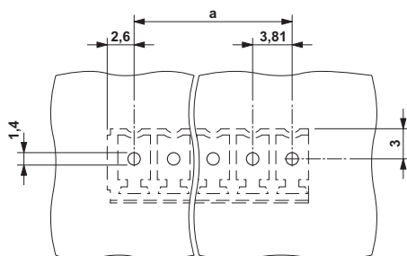
Drilling diagram
