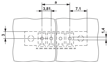
Drilling diagram
