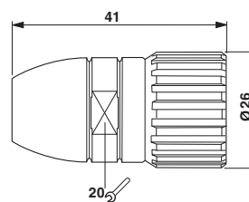
Dimensioned drawing
