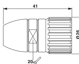
Dimensioned drawing
