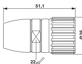
Dimensioned drawing
