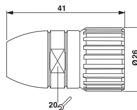
Dimensioned drawing
