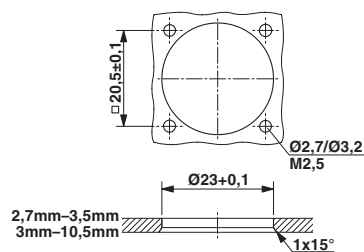
Dimensioned drawing
