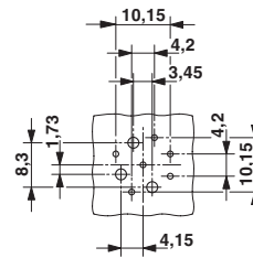
Drilling diagram
