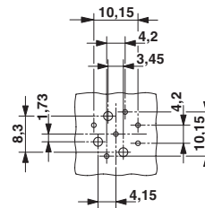
Drilling diagram
