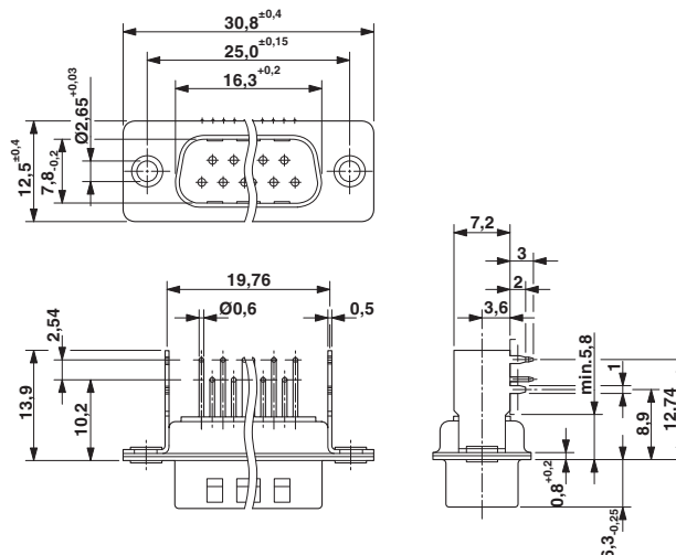
Dimensioned drawing
