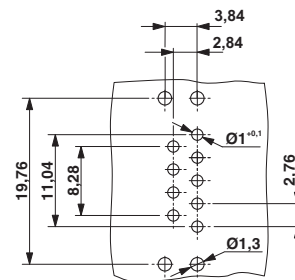
Drilling diagram
