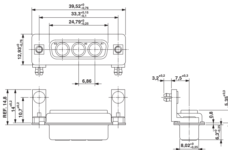
Dimensioned drawing
