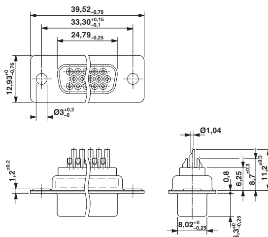
Dimensioned drawing
