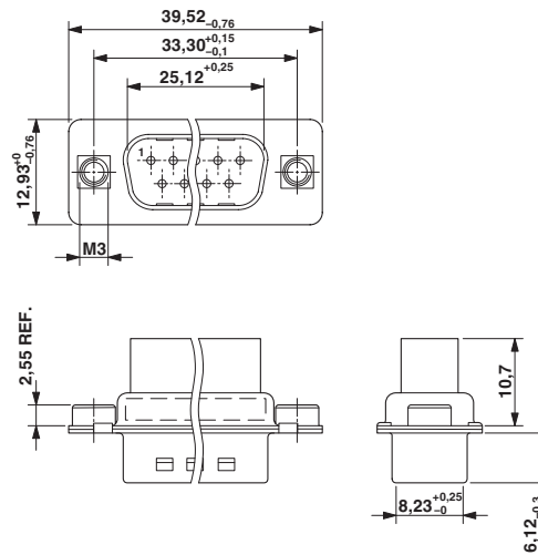
Dimensioned drawing
