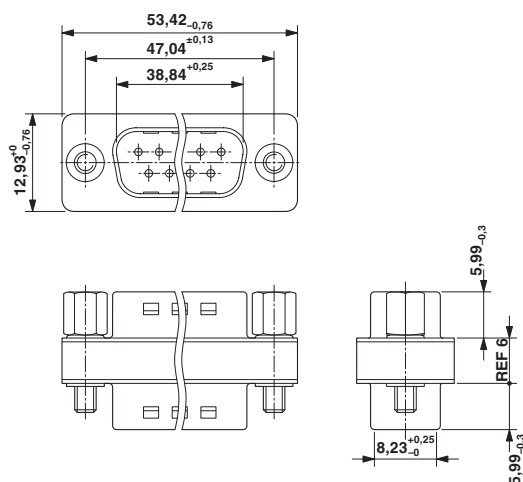
Dimensioned drawing
