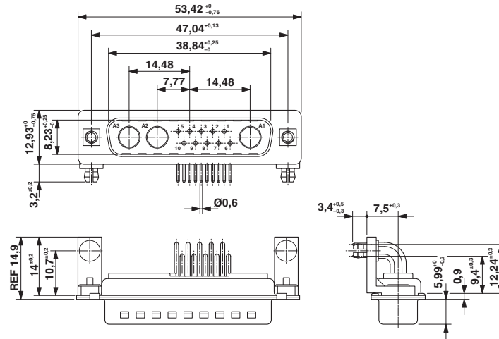
Dimensioned drawing
