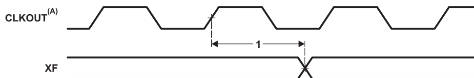
Figure 5-21. XF Timings
