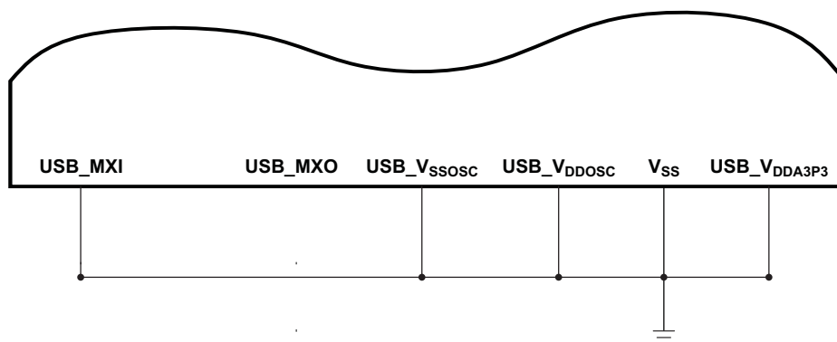
Figure 5-12. Connections when USB Oscillator is Permanently Disabled
