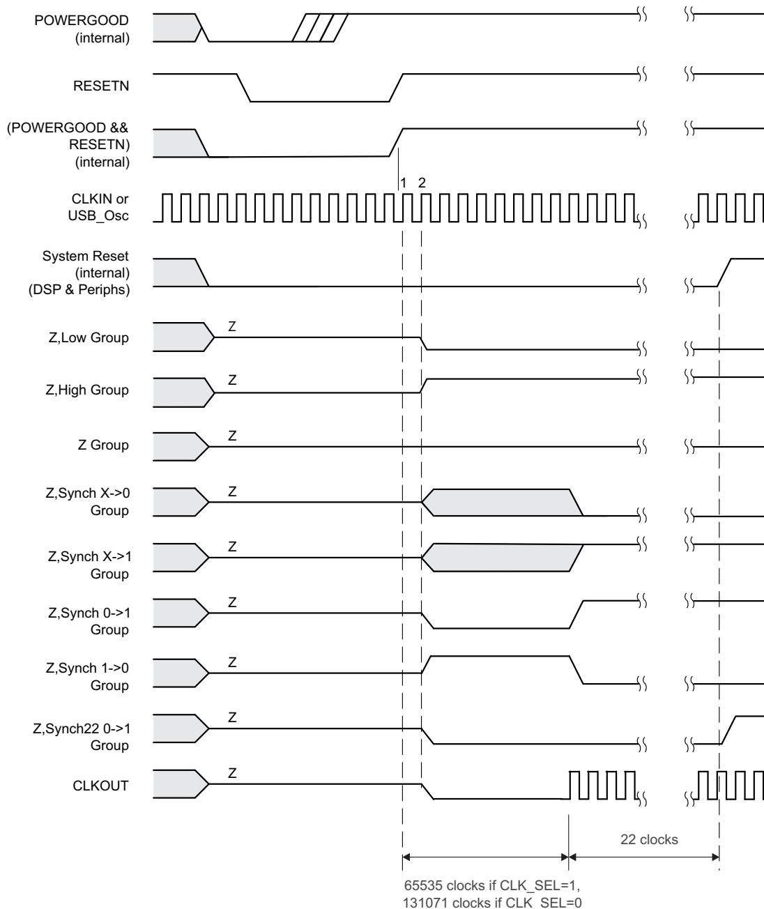
Figure 5-6. Reset Timing When DSP_LDO_EN = 0
