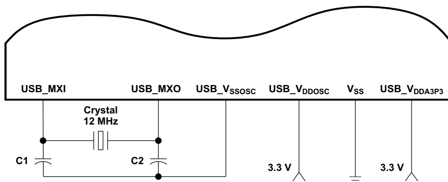
Figure 5-11. 12-MHz USB Oscillator
