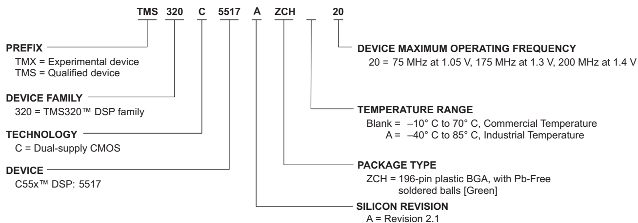
Figure 7-1. Device Nomenclature
