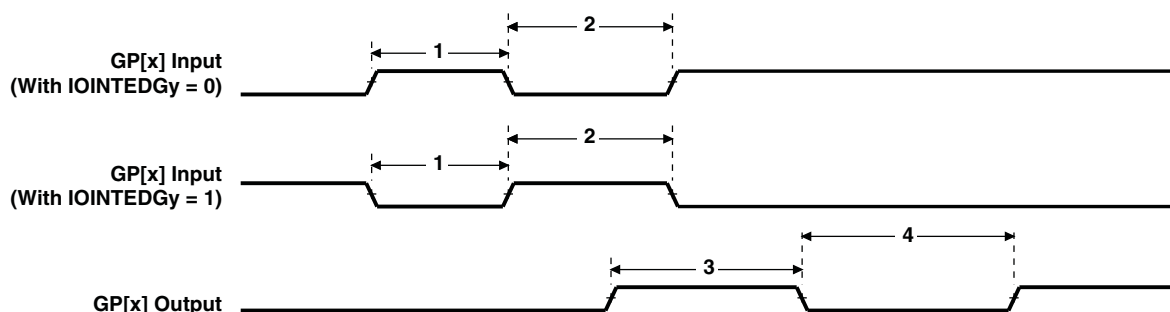
Figure 5-28. GPIO Port Timing
