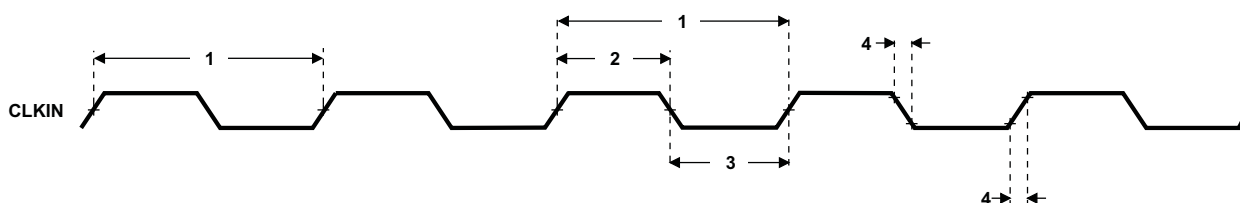
Figure 5-17. CLKIN Timing
