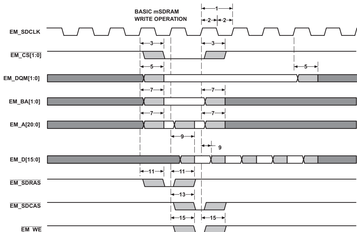
Figure 5-22. EMIF Basic SDRAM and mSDRAM Write Operation
