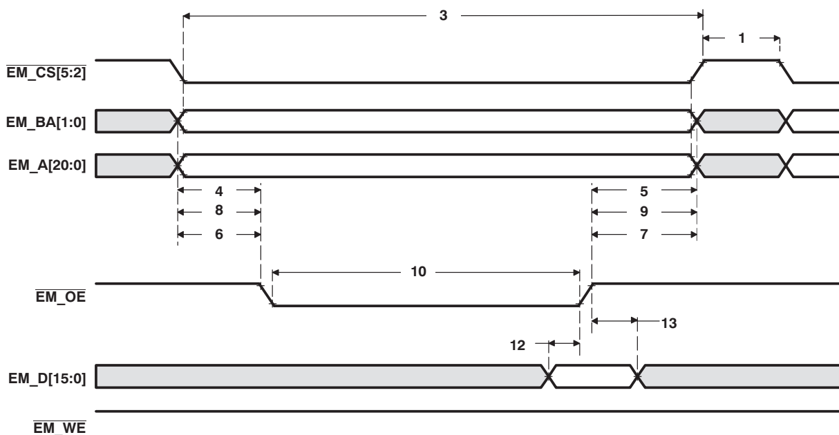
Figure 5-24. Asynchronous Memory Read Timing for EMIF
