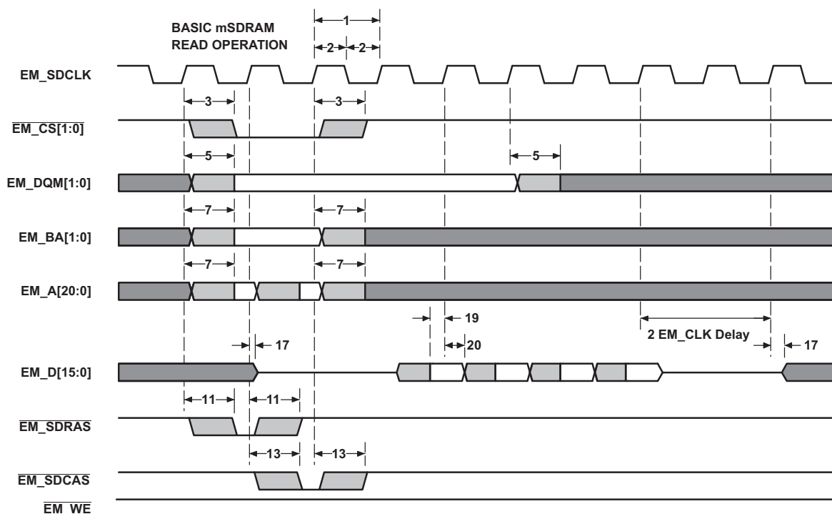
Figure 5-23. EMIF Basic SDRAM and mSDRAM Read Operation
