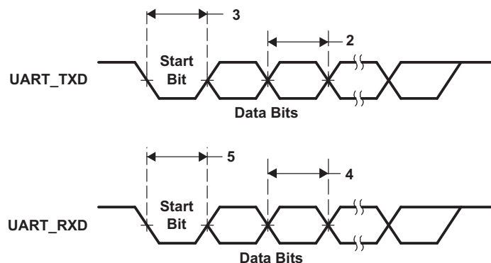
Figure 5-44. UART Transmit and Receive Timing
