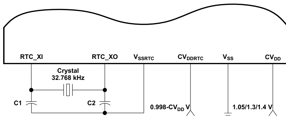
Figure 5-13. 32.768-kHz RTC Oscillator
