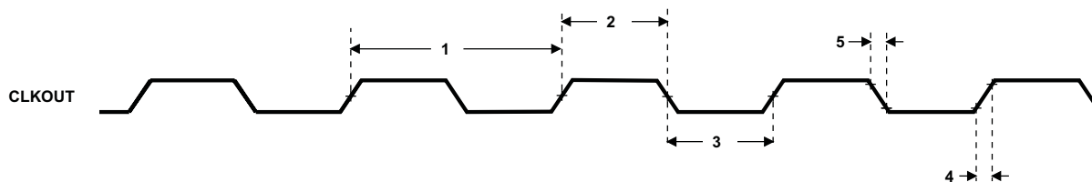
Figure 5-18. CLKOUT Timing
