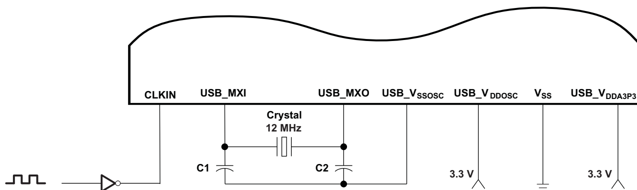
Figure 5-15. LVCMOS-Compatible Clock Input With USB Oscillator Enabled
