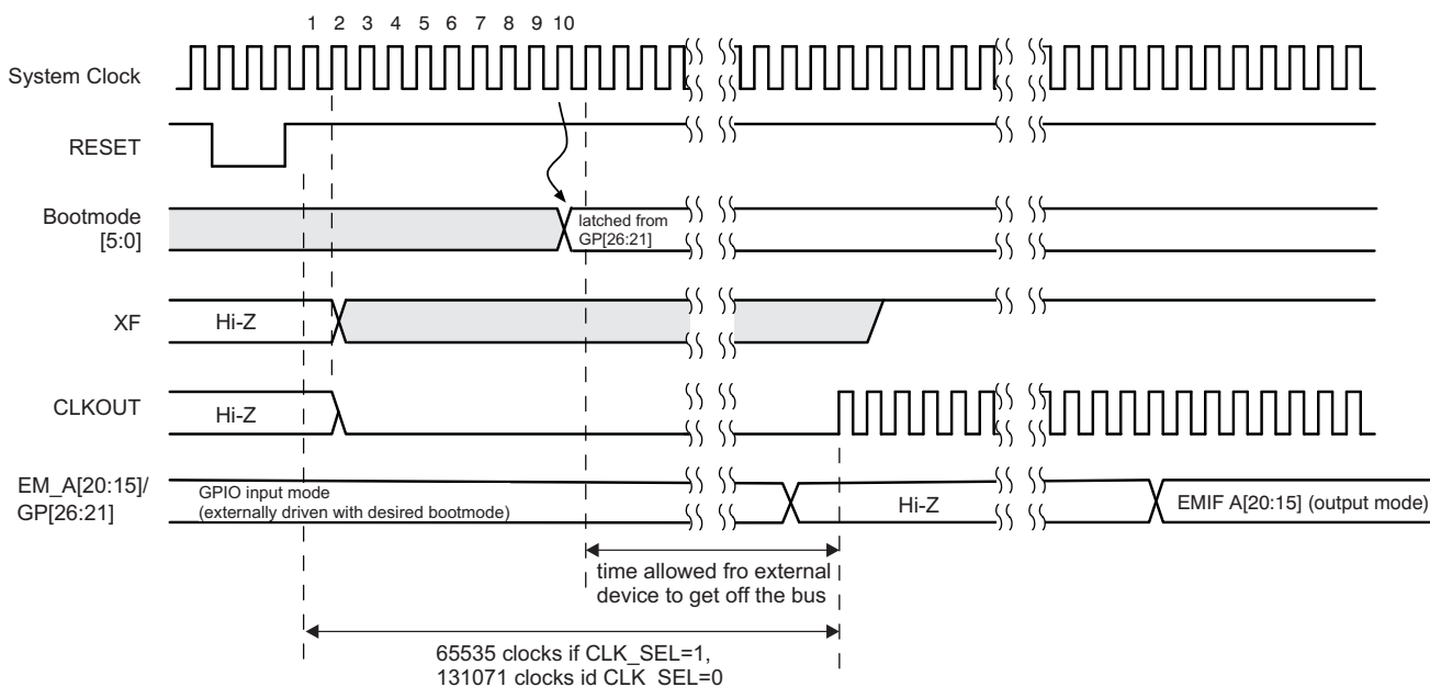
Figure 5-9. BootMode Latching
