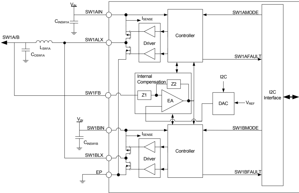
Figure 11. SW1A/B Single Phase Block Diagram
