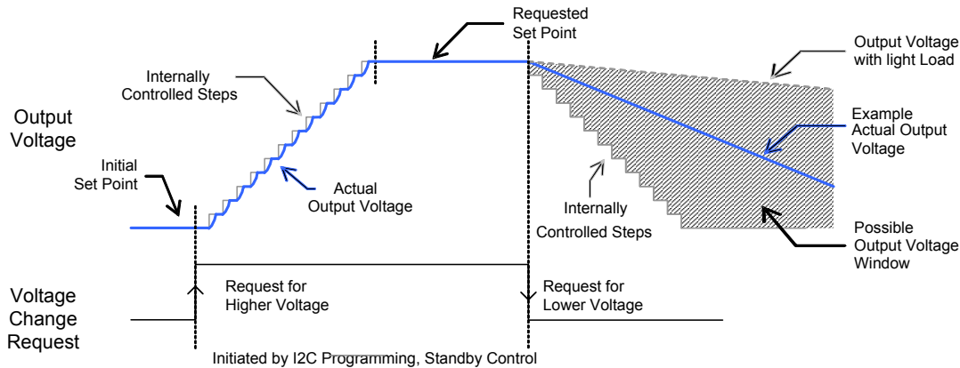
Figure 10. Voltage Stepping with DVS
