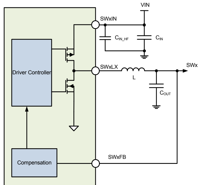
Figure 26. Generic Buck Regulator Architecture
