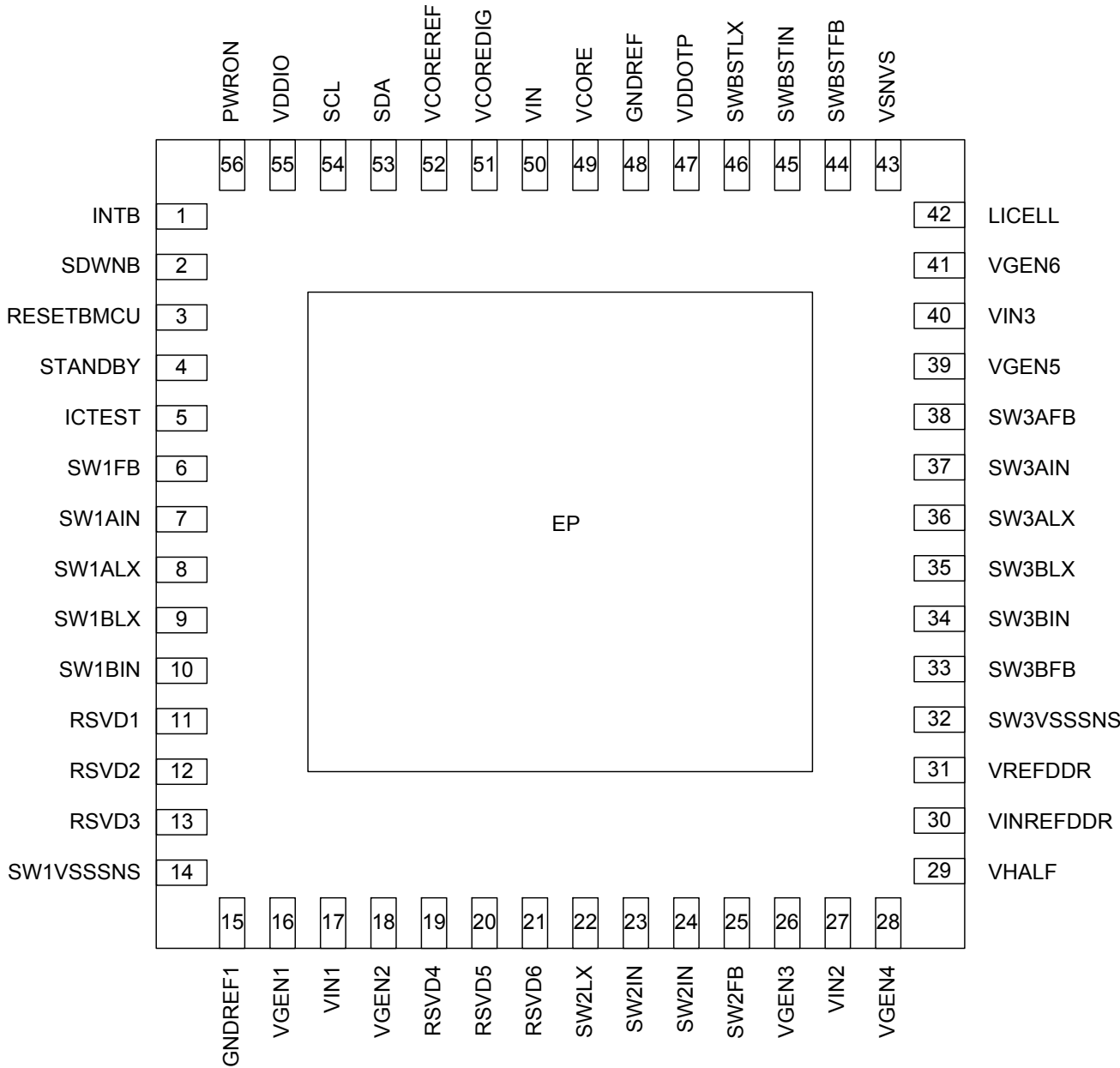
Figure 3. Pinout Diagram
