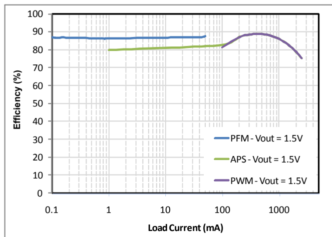
Figure 17. SW3AB Single Phase Efficiency Waveforms
