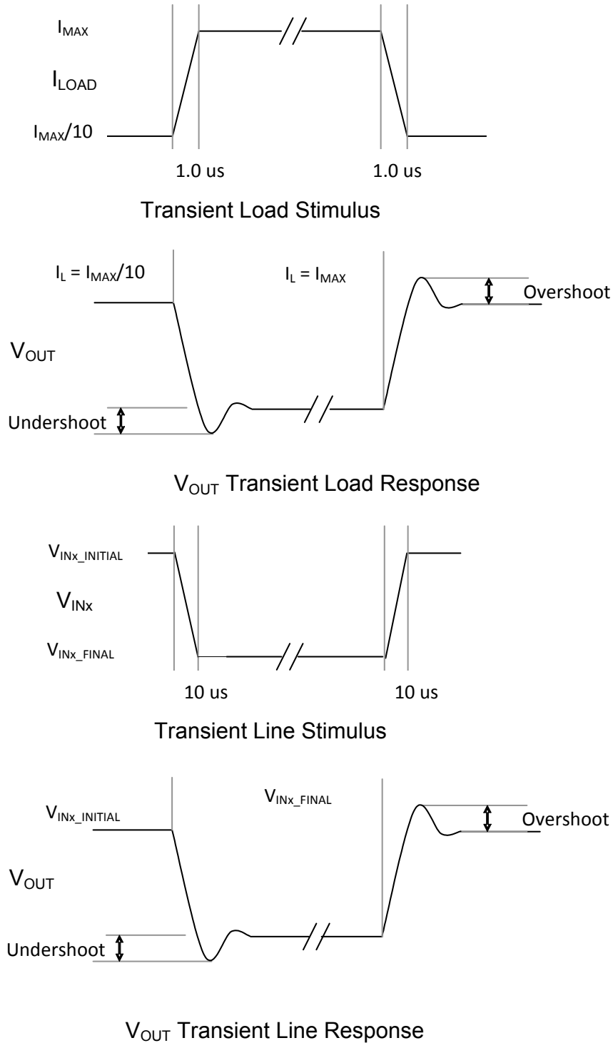
Figure 20. Transient Waveforms
