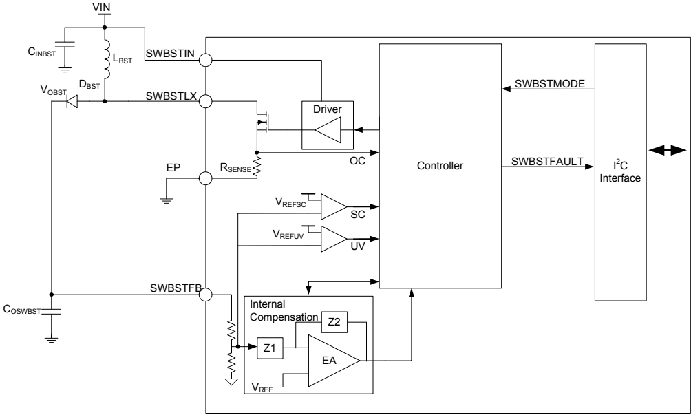
Figure 18. Boost Regulator Architecture
