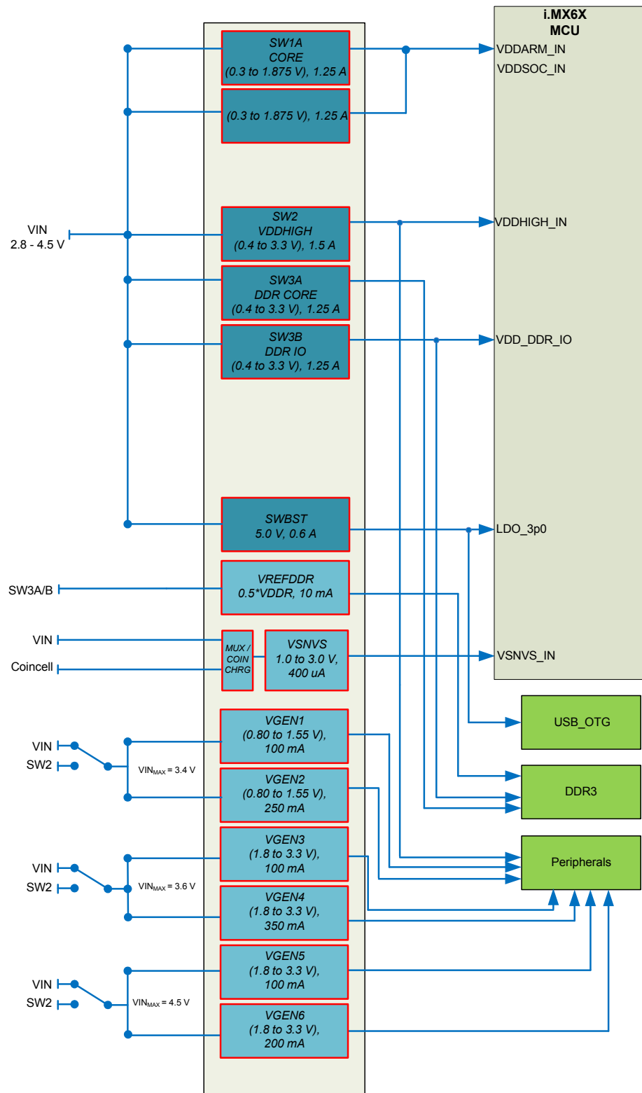
Figure 9. PF0200 Typical Power Map
