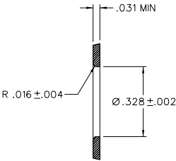
MOUNTING HOLE DETAIL
