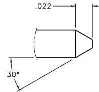
POINTING DETAIL 20:1
