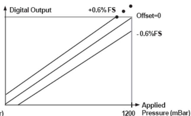
Figure 4.4—Custom Offset (Z=) Options
