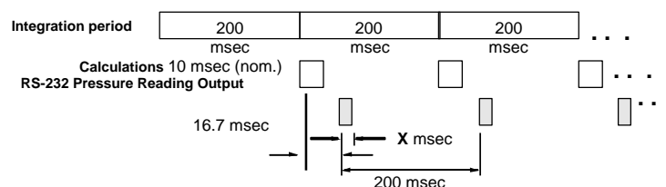
Figure 7.2—Default Continuous Pressure Reading Timing Diagram
