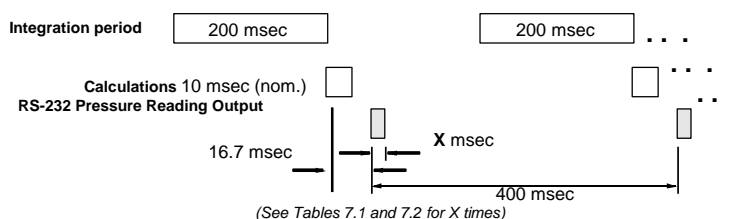
Figure 7.3—Continuous Pressure (with IC = 1) Timing Diagram
