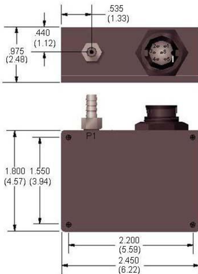
Figure 9.1—HPB Case Outline Standard
