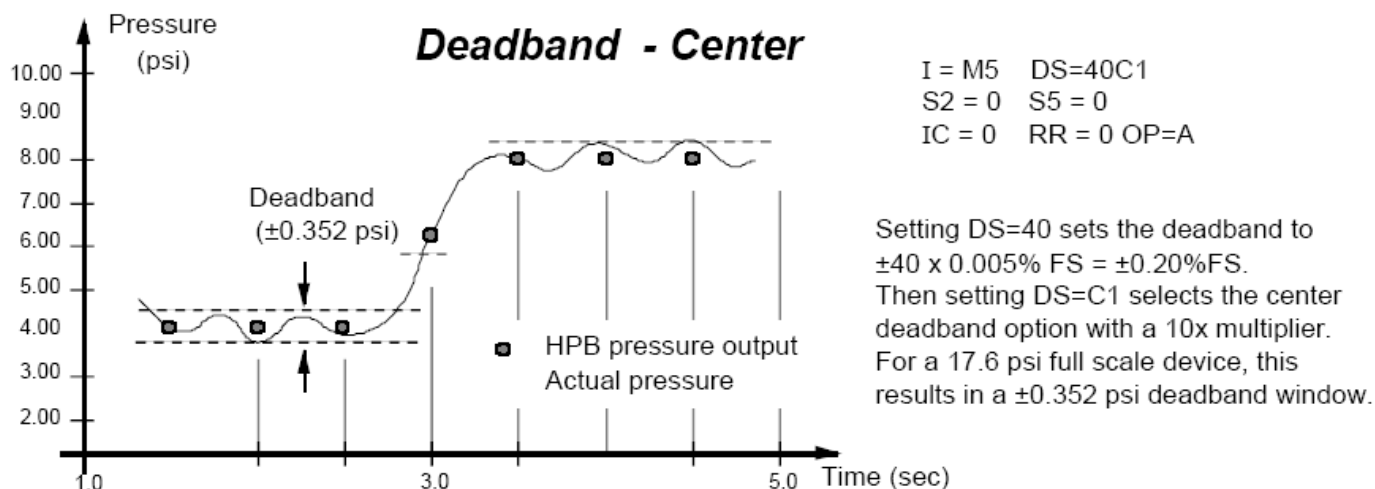
Figure 4.9a-Deadband and Sensitivity (DS) Command Examples
