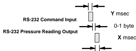
Figure 7.1—Default Single Pressure Reading Timing Diagram
