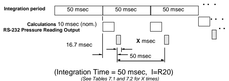
Figure 7.4—Timing Diagram for 20 Readings Per Second
