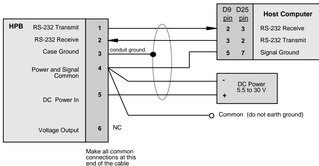
Figure 6.2—Connection for RS-232 Operation
