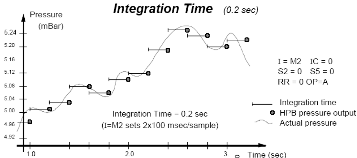
Figure 4.5—Integration (I=) Command, Example 1
