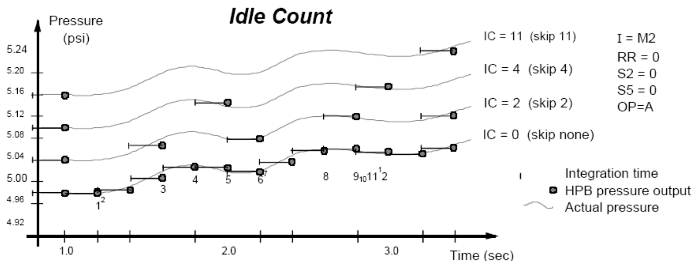
Figure 4.10—Idle Count (IC) Command Example
