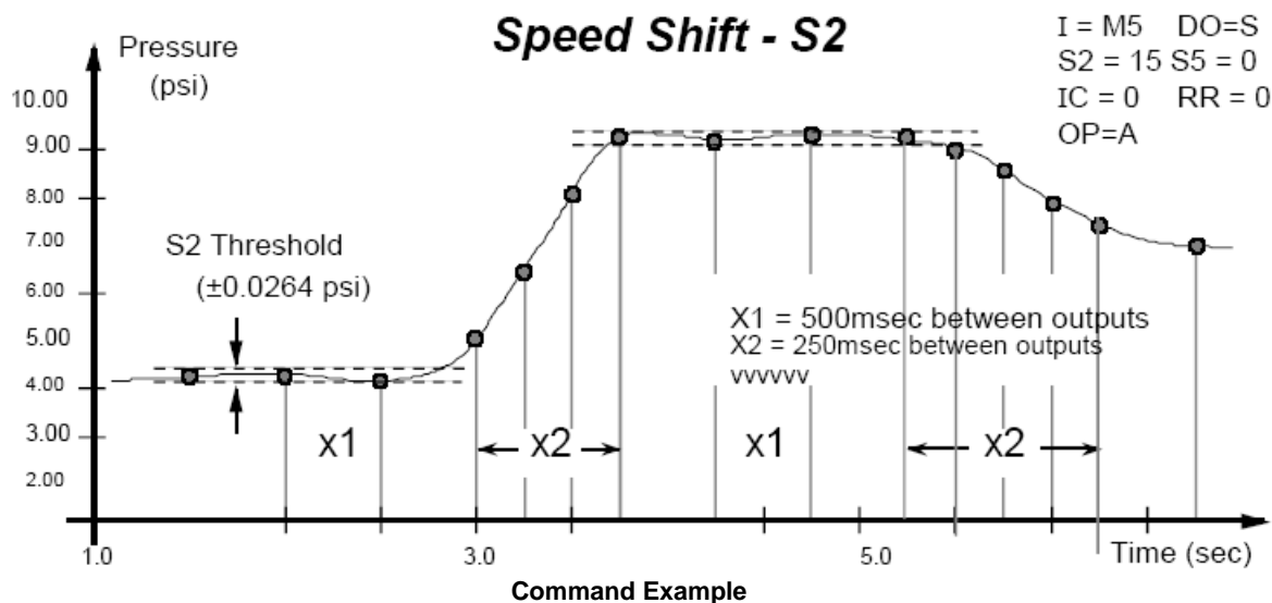
Figure 4.7—S2 Speed Shift
