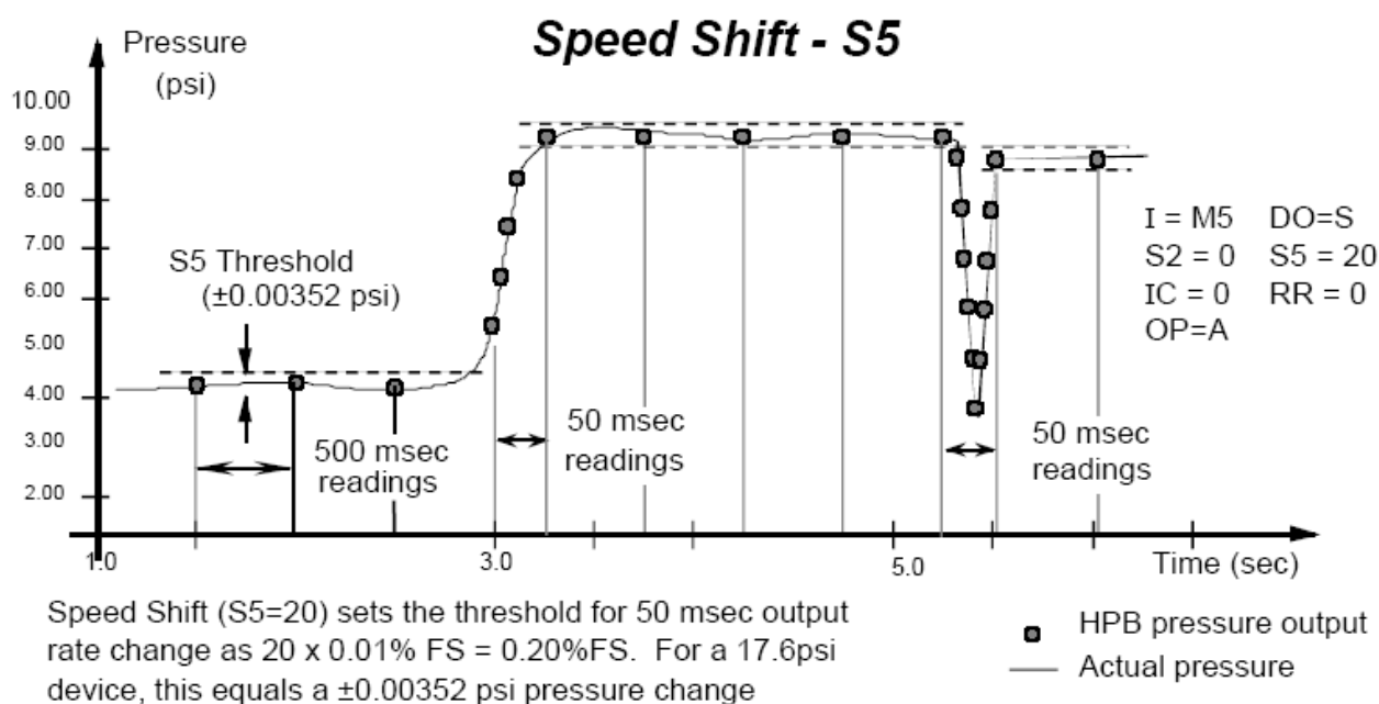
Figure 4.8—S5 Speed Shift Command Example
