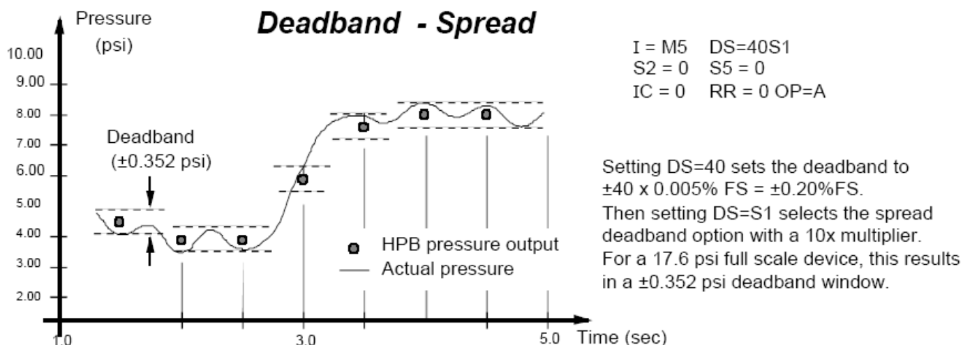
Figure 4.9b—Deadband and Sensitivity (DS) Command Examples
