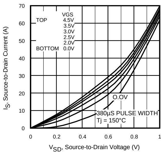
Fig 8. Typical Reverse Output Characteristics
