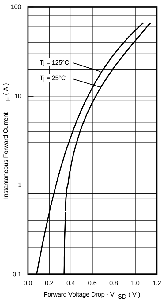
Fig. 11 - Typical Forward Voltage Drop Characteristics
