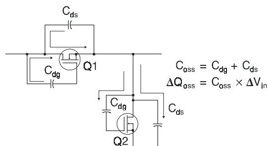
Figure 2: Q_{oss} Characteristic
