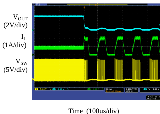
Figure 12. Short Circuit Protection ( I_{OUT}=1\text{A} )
