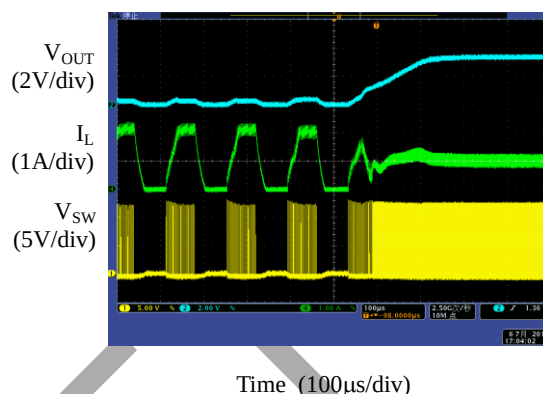
Figure 13. Short Circuit Recovery ( I_{OUT}=1\text{A} )
