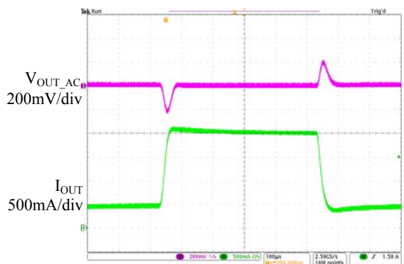
Time 100µs/div
