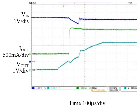
Figure 25. Leave OVP Function ( V_{IN}=6V to 5V )
