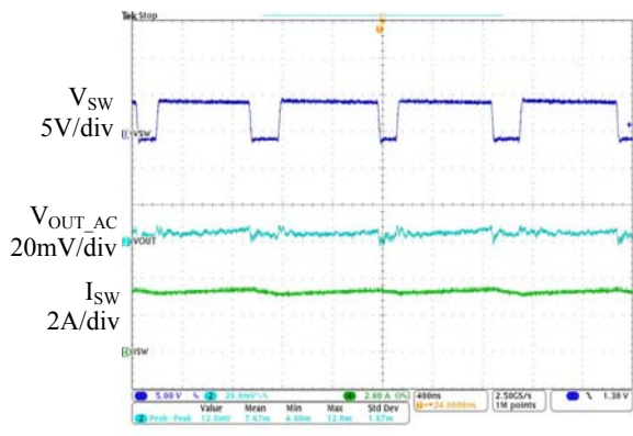
Time 400ns/div
