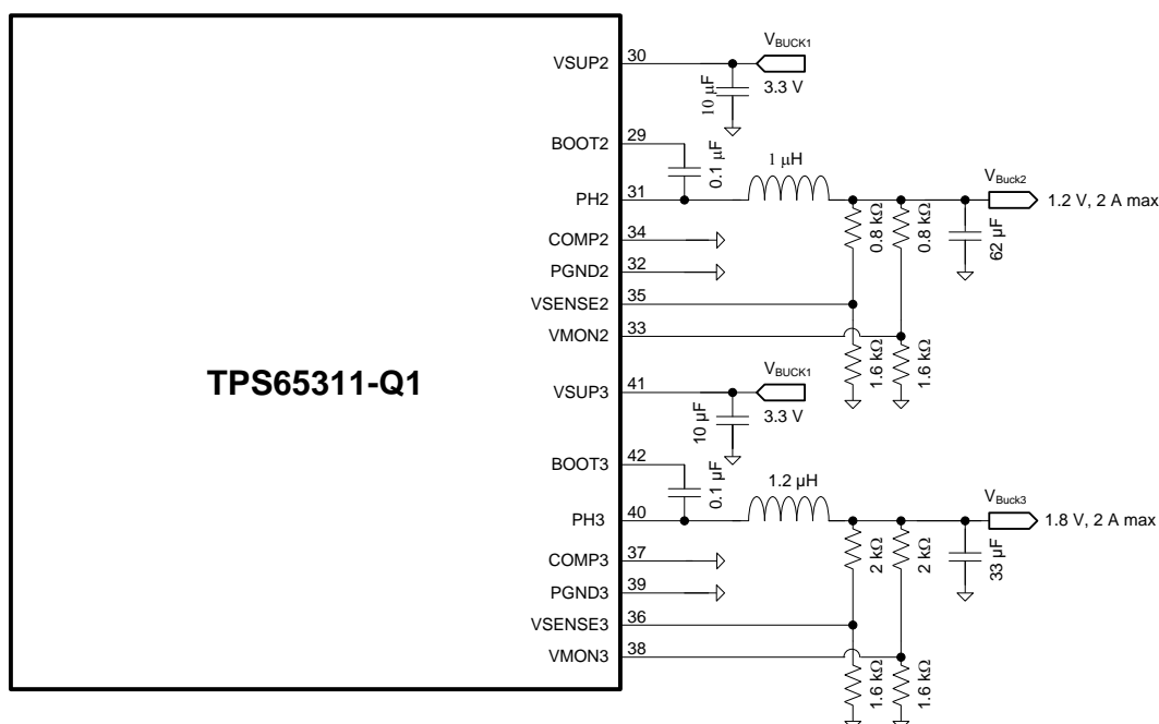
Figure 28. Synchronous Buck Converter Schematic
