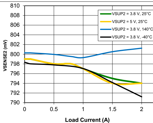
Figure 3. Load Regulation BUCK2 = 3.3 V EXTSUP Pin Open
