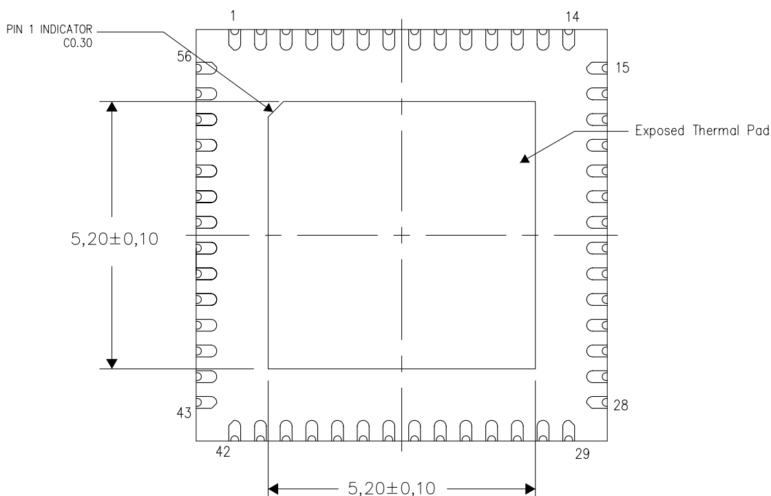
Bottom View
