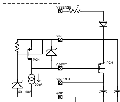
Figure 20. PMOS Control Circuitry
