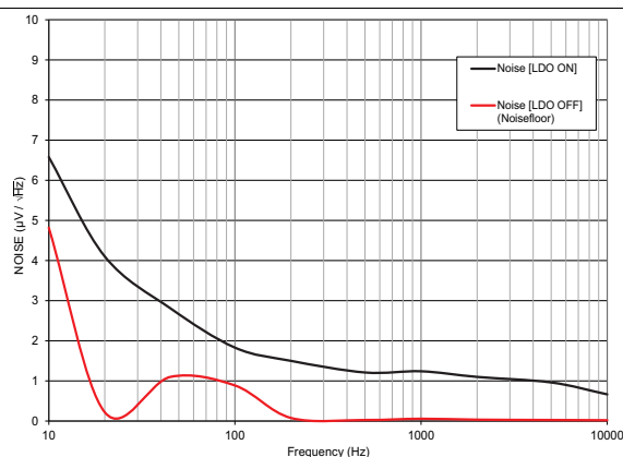
Figure 14. LDO Noise Density
