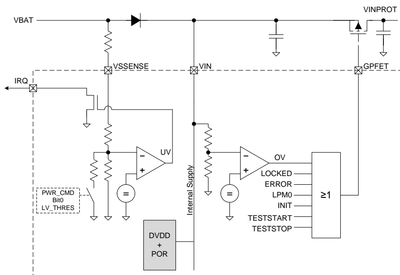
Figure 19. Overvoltage or Undervoltage Detection Circuitry
