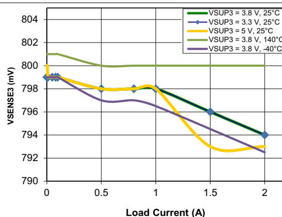
Figure 4. Load Regulation BUCK3 = 1.2 V EXTSUP Pin Open
