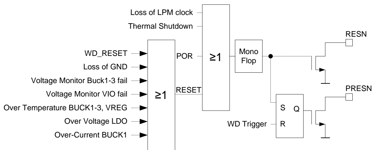
Figure 17. RESET Functionality
