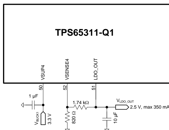
Figure 38. Linear Regulator Schematic
