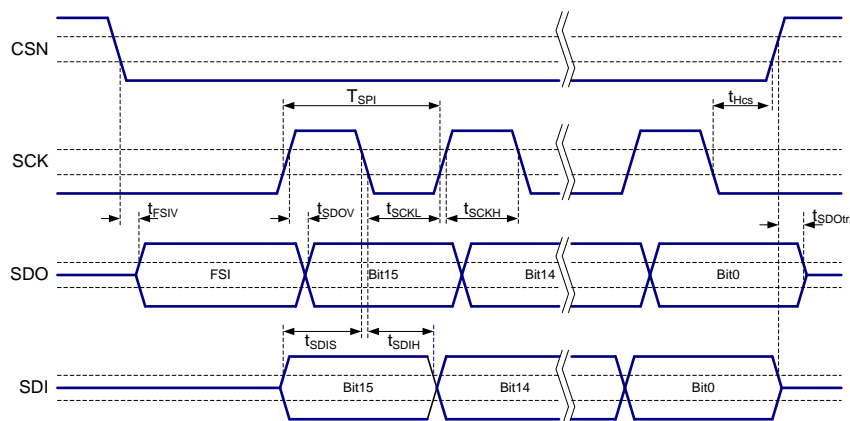
Figure 1. SPI Timing
