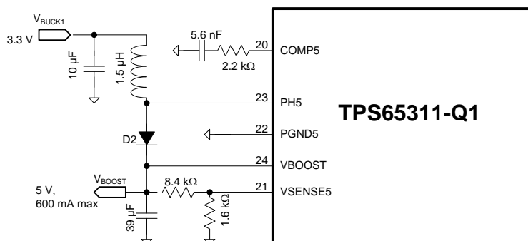
Figure 35. BOOST Converter Schematic
