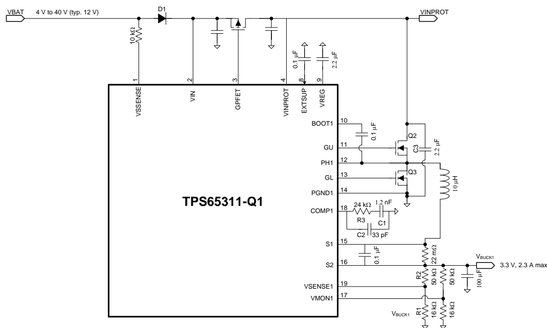
Figure 26. Buck Controller Schematic
