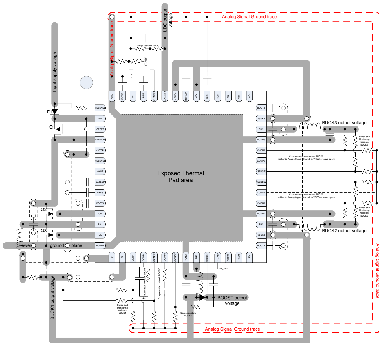
Figure 41. TPS65311-Q1 Layout Example
