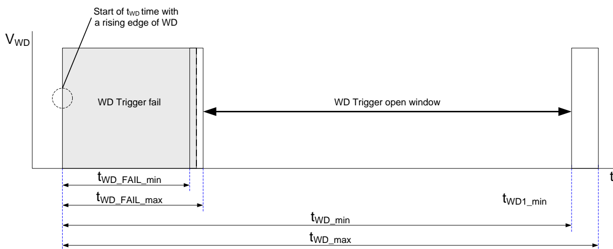
Figure 23. WD Window Description
