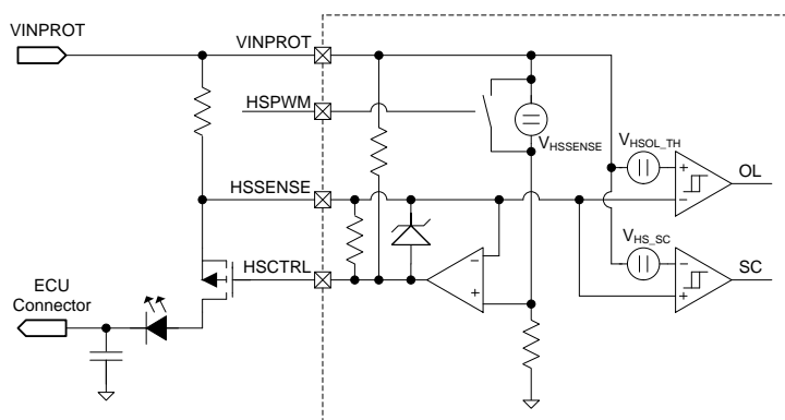
Figure 21. High-Side Control Circuit
