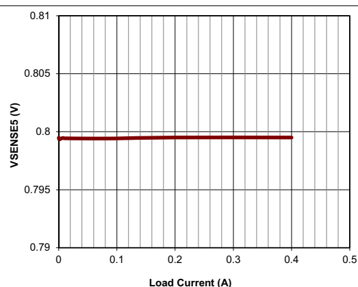
Figure 12. Load Regulation BOOST = 5 V AT 25°C EXTSUP Pin Open, BOOST Supply Input = 3.8 V
