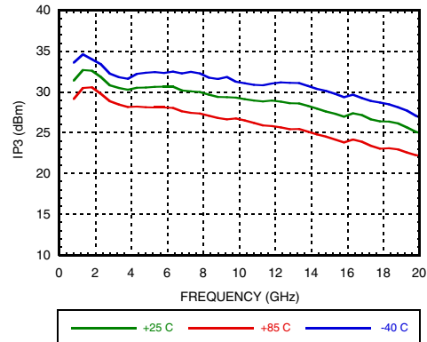
Output IP3 vs. Temperature [1]
