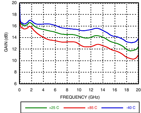
Gain vs. Temperature [1]
