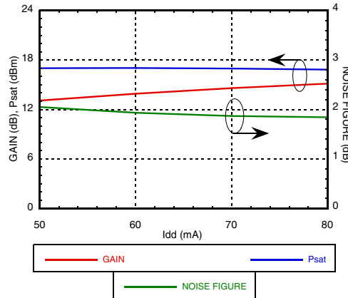
Noise Figure, Gain & Power vs. Supply Current @ 12 GHz
