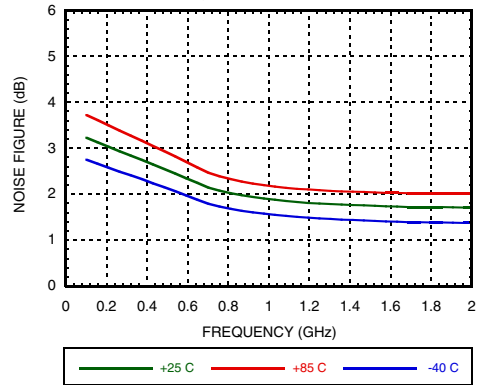
Noise Figure vs. Temperature, Low Frequency
