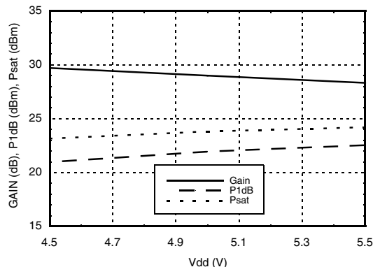
Gain & Power vs. Supply Voltage @ 11 GHz
