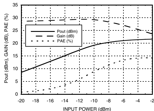
Power Compression @ 17 GHz
