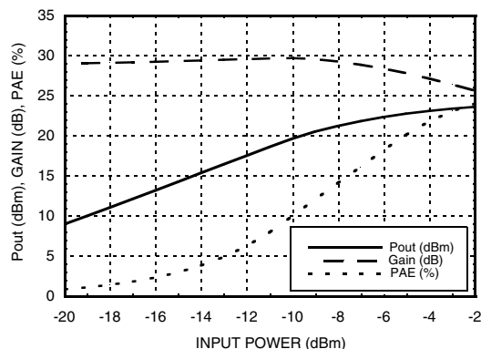
Power Compression @ 11 GHz
