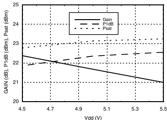
Gain & Power vs. Supply Voltage @ 12.5 GHz
