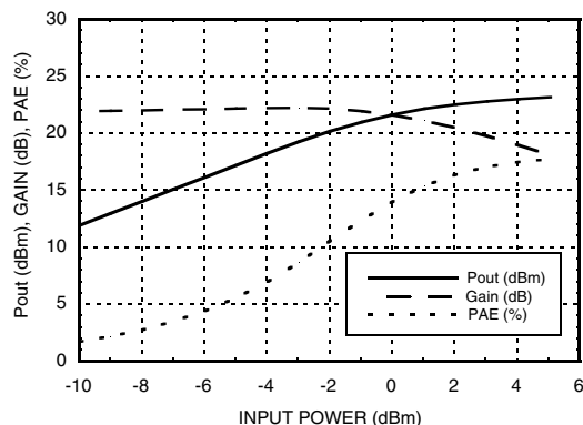
Power Compression @ 12.5 GHz
