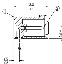
SECTION Z-Z
