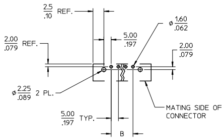
⑧ PCB LAYOUT
