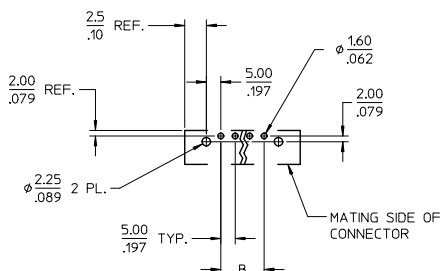
② PCB LAYOUT
