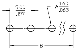
PTH LAYOUT
