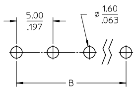
PTH LAYOUT
