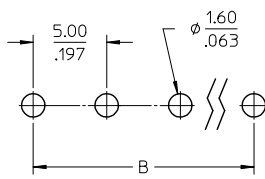
PTH LAYOUT
